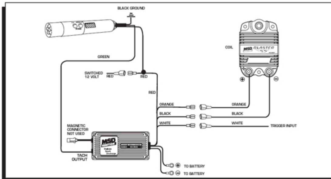
Figure 2 Installing with an MSD Ignition.
