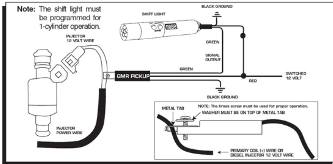
Figure 7 Installation to a Diesel Injector.
