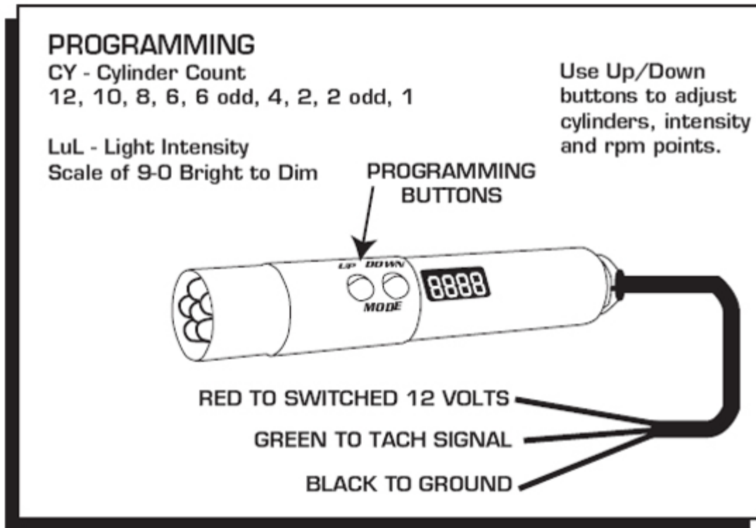
Figure 1 Digital Shift Light Wiring and Programming.
