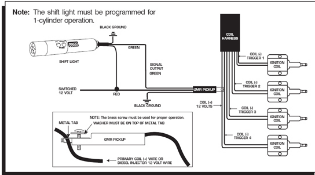
Figure 3 Installation on an Inductive Coil-Per-Cylinder Ignition System.
