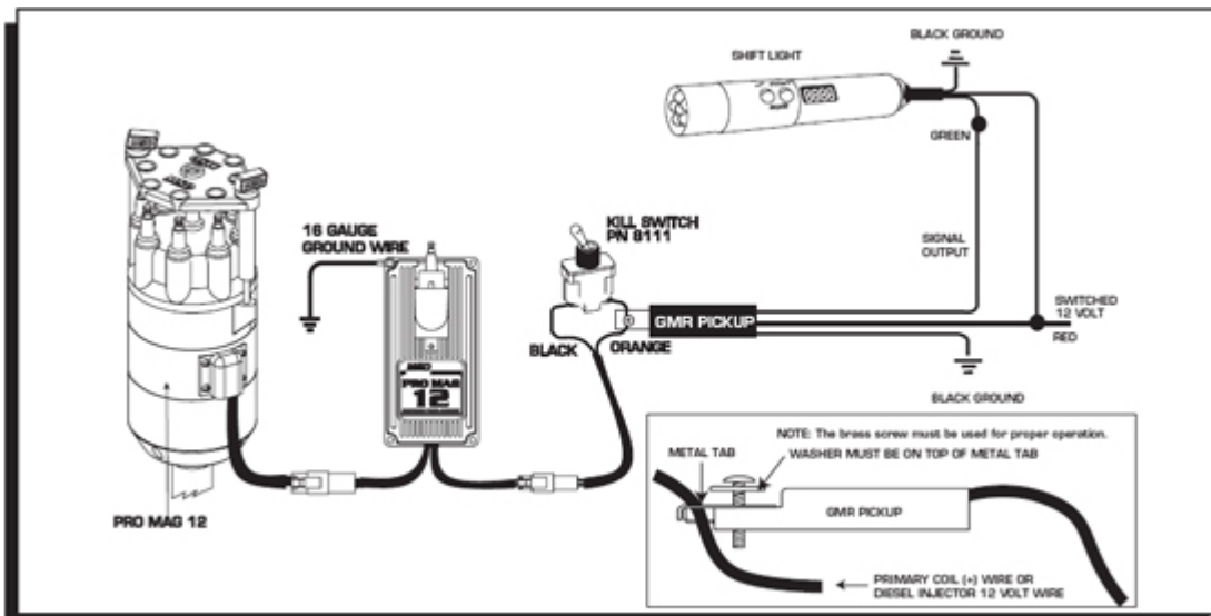
Figure 6 Wiring the 12 Amp Pro Mag.
