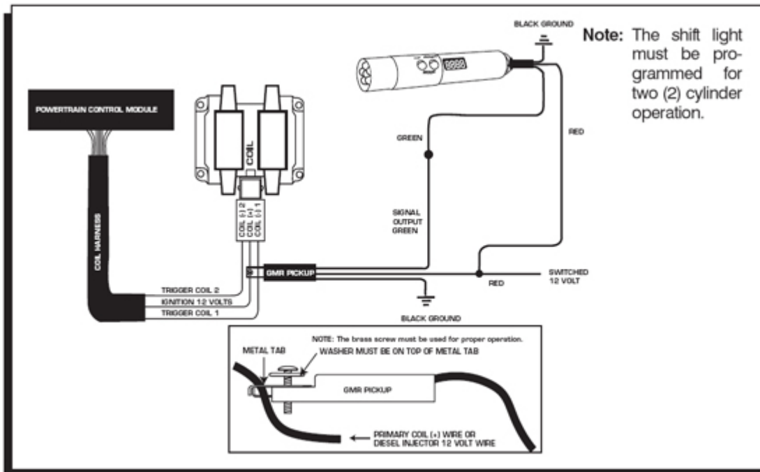
Figure 4 Installing to an Inductive Coil Pack.
