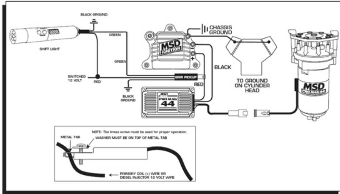
Figure 5 Wiring the Pro Mag 44 Electronic Points Box.
