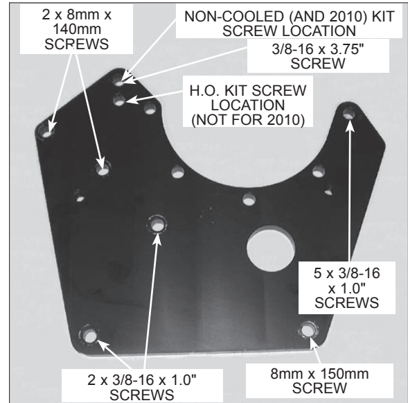
Fig. 6.2-a (Non-Cooled Kit Screw Location MUST be used for 2010 H.O. Kit)
