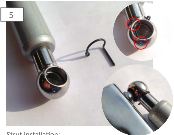
Strut installation: Remove the retaining clip. Place strut on the ball stud. Then reinstall the retaining clip. **Note: Make sure the retaining clip slides all the way through.
